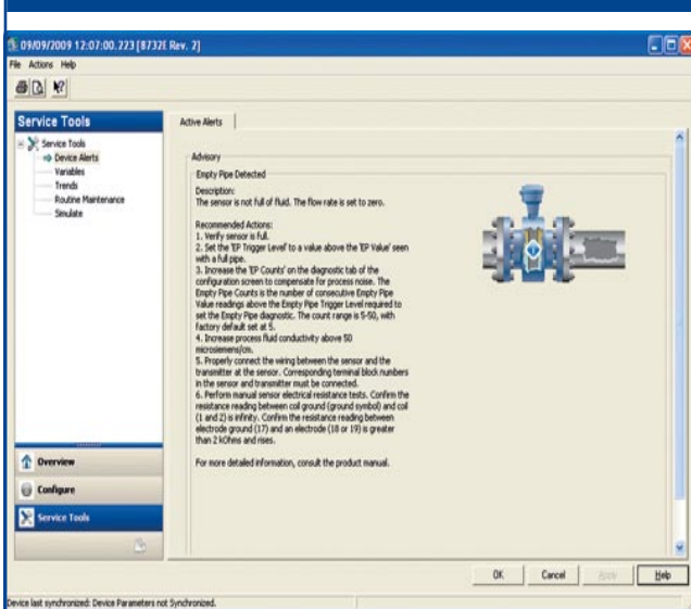
Figure 6: Magnetic flowmeter diagnostics page with actionable help made available through EDDL.
