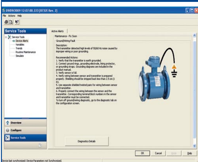
Figure 4: Magnetic flowmeter diagnostics page with actionable help provided by manufacturer's expert.
