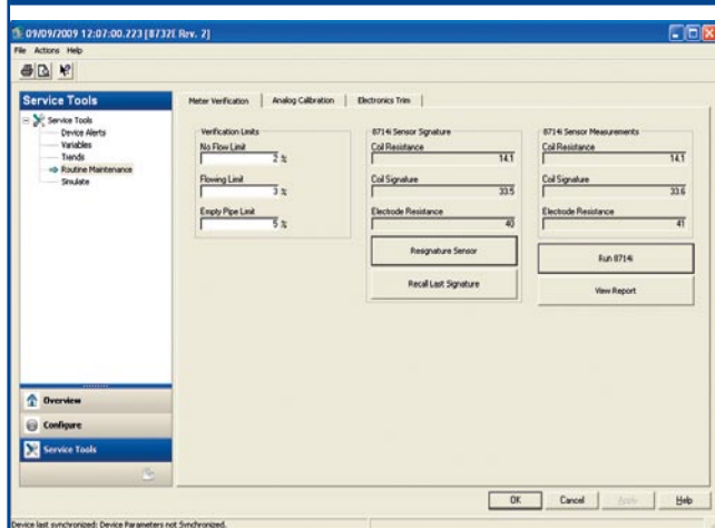
Figure 2: Meter verification detects leading indicators of drift by comparing present characteristics against stored baseline signature.
