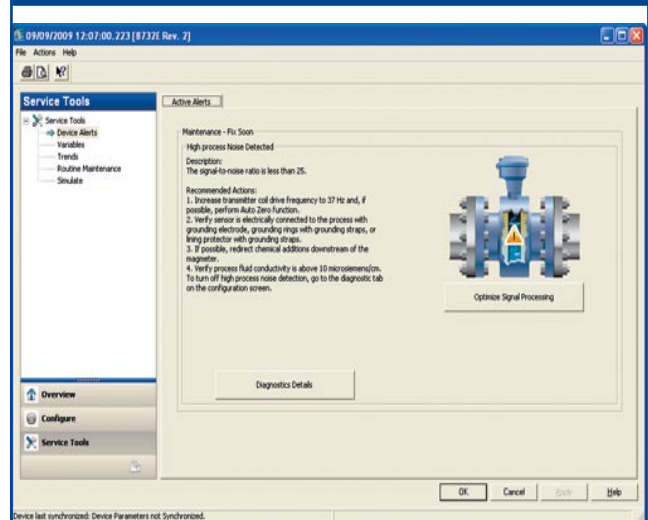
Figure 5: Magnetic flowmeter diagnostics page with know-how provided by manufacturer's expert as help text and illustrations.
