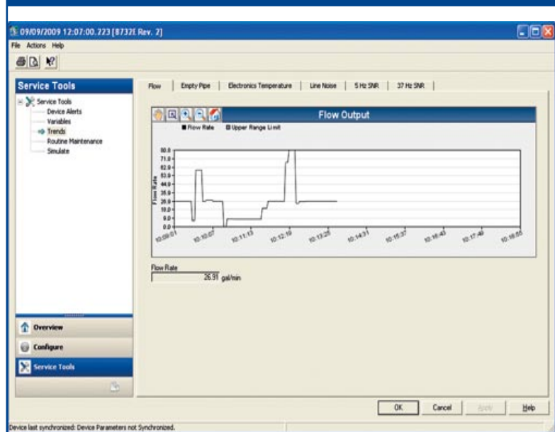
Figure 8: EDDL enhancements include multi-pen trend chart that assists in identifying intermittent problems.
